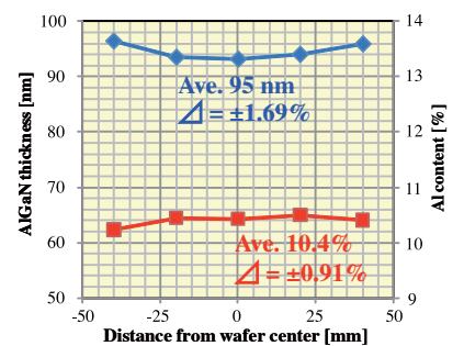
Thickness & Al comp. distribution of un-AlGaN
