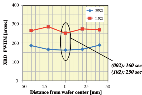
XRD FWHM of un-GaN
