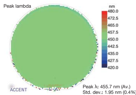
PL peak wavelength mapping of MQW sample
